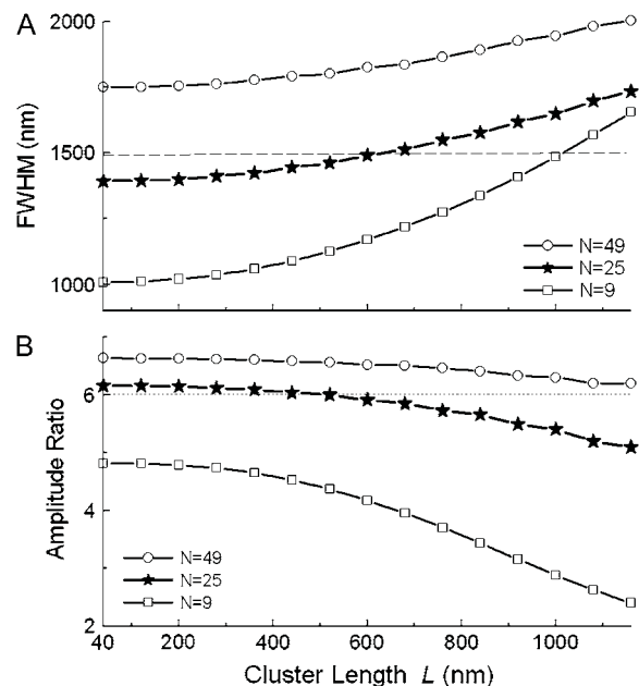
FIGURE 6 Effects of changing cluster dimensions (length L ) on puff FWHM at time T_2 ( A ) and the amplitude ratio R between puff and trigger ( B ). Clusters containing 49 ( \circ ), 25 ( \star ), and 9 ( \square ) open channels were simulated. For comparison, the dashed lines in A and B show, respectively, the mean FWHM ( W_0 = 1500 nm) and the amplitude ratio ( R_0 = 6 ) of averaged experimental puffs.
