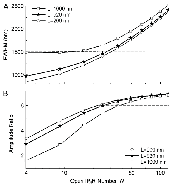
FIGURE 5 Effects of changing open IP 3 R number N on puff width at time T_2 ( A ), and on the amplitude ratio R between puff and trigger ( B ). Different clusters with lengths L = 200 nm ( \circ ), 520 nm ( \star ), and 1000 nm ( \square ) were simulated. For comparison, the dashed lines in A and B show the mean FWHM ( W_0 = 1500 nm) and amplitude ratio ( R_0 = 6 ) of experimental observations of puffs.
