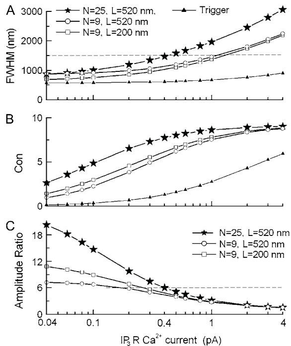
FIGURE 7 Influence of IP 3 R channel Ca 2+ current on puff FWHM at time T_2 (A), confocal image amplitude (B), and the amplitude ratio R between puff and trigger (C). Three different clusters are considered: open channel number N = 25 and cluster length L = 520 nm (★); N = 9 , and L = 520 nm (○); and N = 9 and L = 200 nm (□). Additionally, solid triangles show the corresponding relationships for the trigger event at time T_1 . For comparison, the dashed lines in A and C mark, respectively, the FWHM ( W_0 = 1500 nm) and the amplitude ratio ( R_0 = 6 ) of the mean experimental puff.
